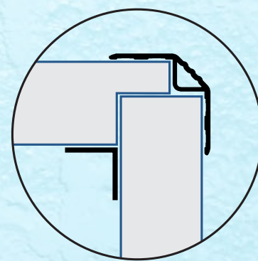
Thermal bridge-free design
